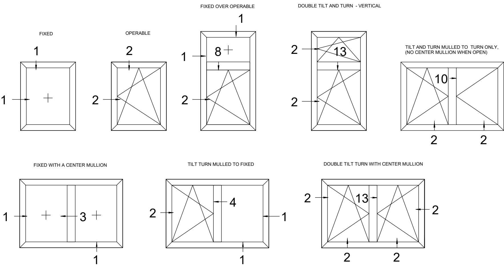
ELEVATIONS - ZOLA THERMO ALU75 PANORAMIC VIEW NOT TO SCALE
