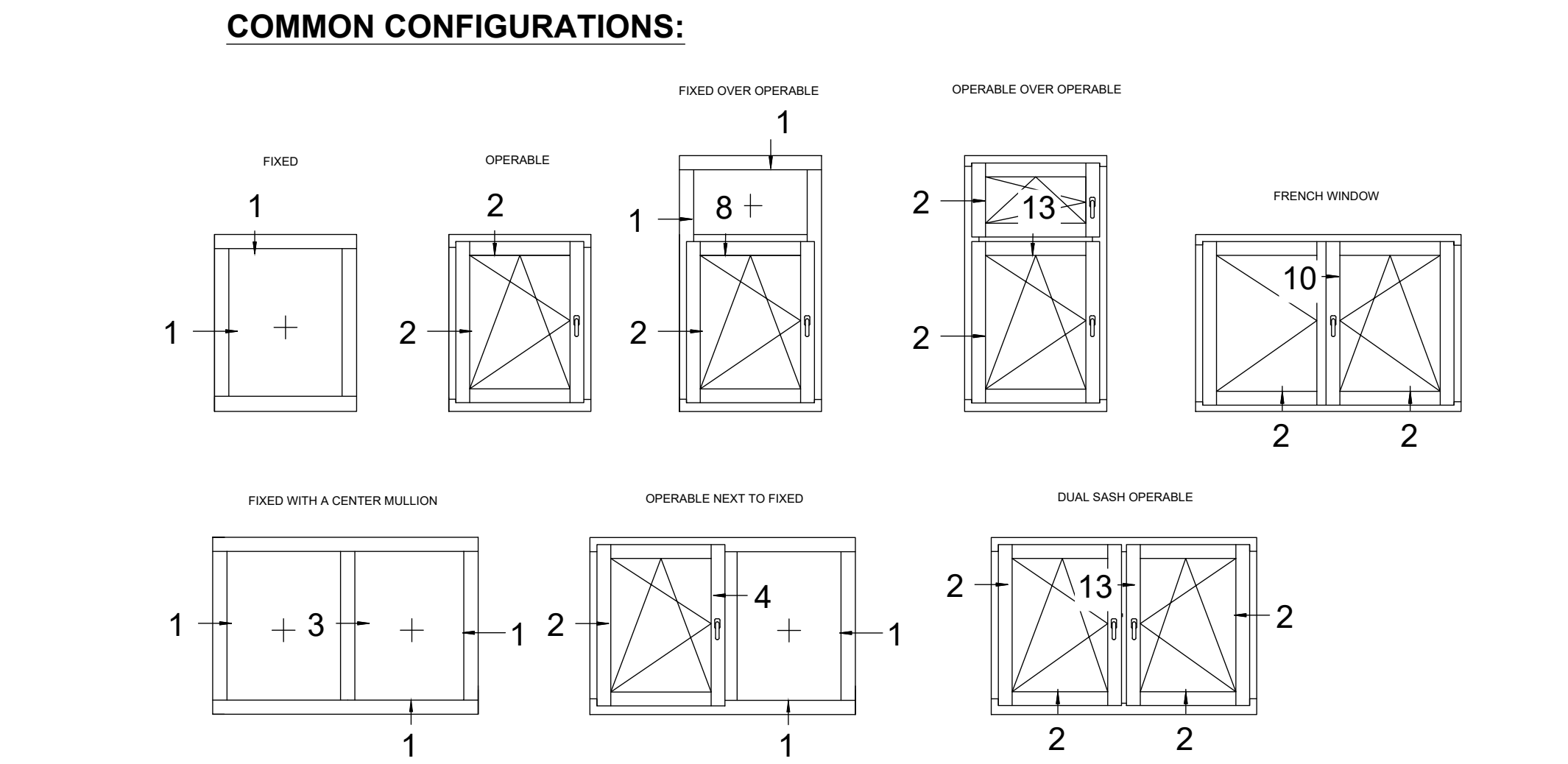
A ELEVATIONS - ZOLA CLASSIC PLUS CLAD SERIES II NOT TO SCALE
